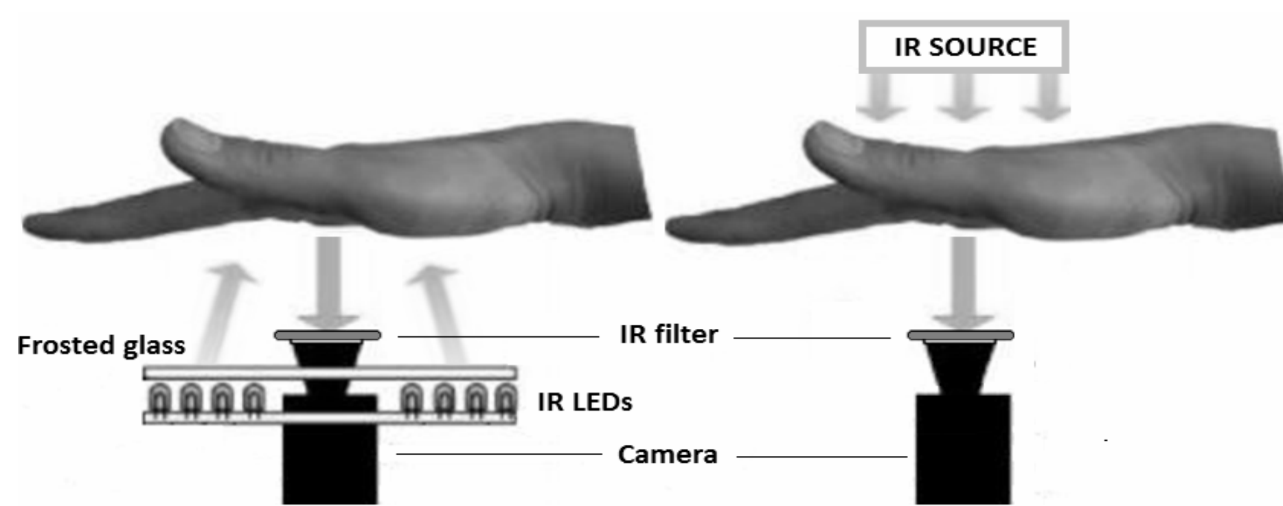
Figure.5: Image acquisition setup for reflection approach (left) and transmission approach (right).
